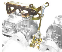
Throttle linkage LP1000 Cable Top Mount for Dual Weber 40 /45/48 DCOE Carburetor
