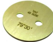
WEBER 40 DCOE/DCOM Throttle plate valve butterfly 79°30'
