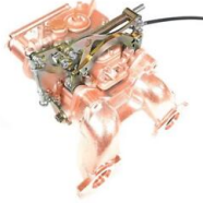
Throttle linkage Left/Right Dual Weber 38/40/45/48 DCOE Carburetors
